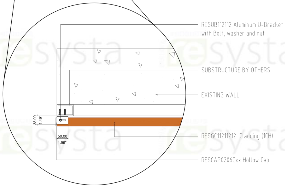
DETAIL - 3.0
