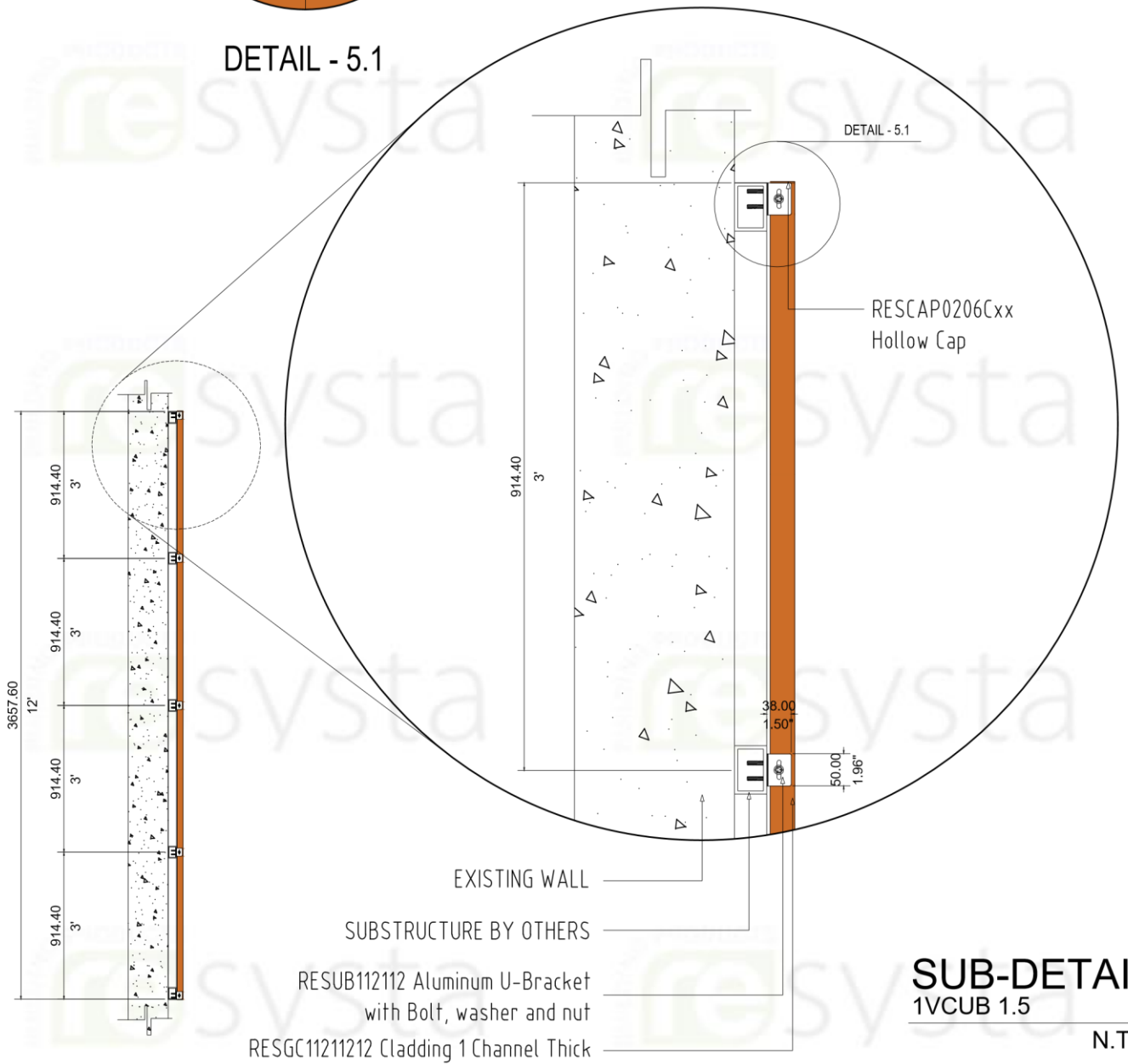
SIDE ELEVATION
