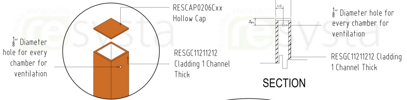
DETAIL - 5.1
