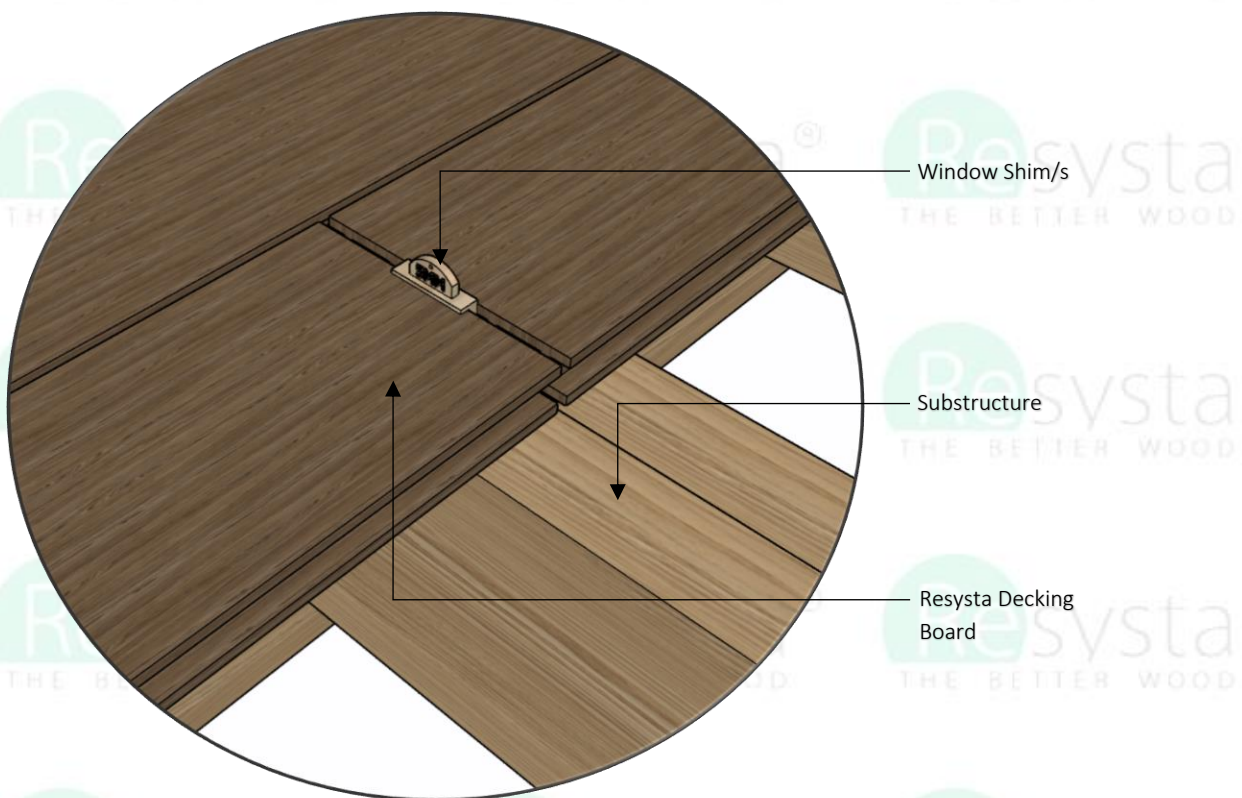
ISOMETRIC VIEW RESYSTA DECKING
