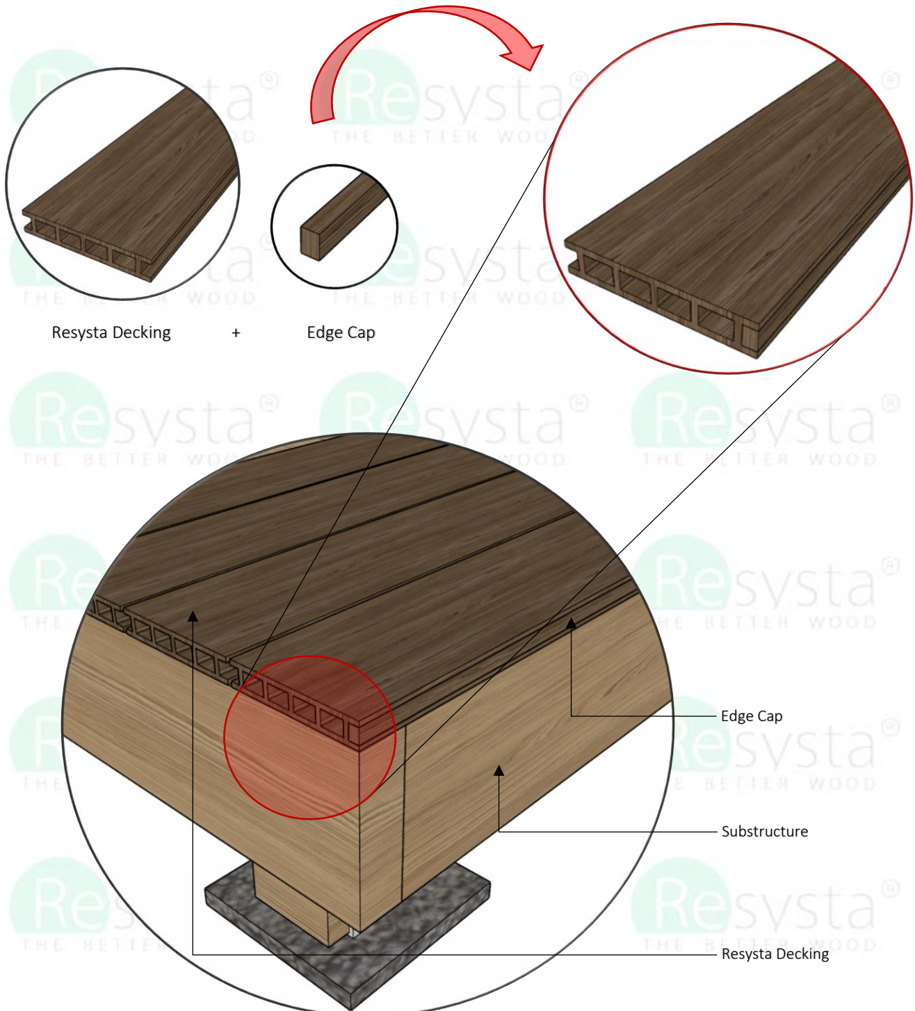
ISOMETRIC VIEW RESYSTA DECKING
