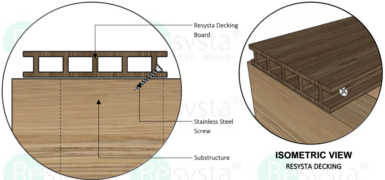
SECTION RESYSTA DECKING
