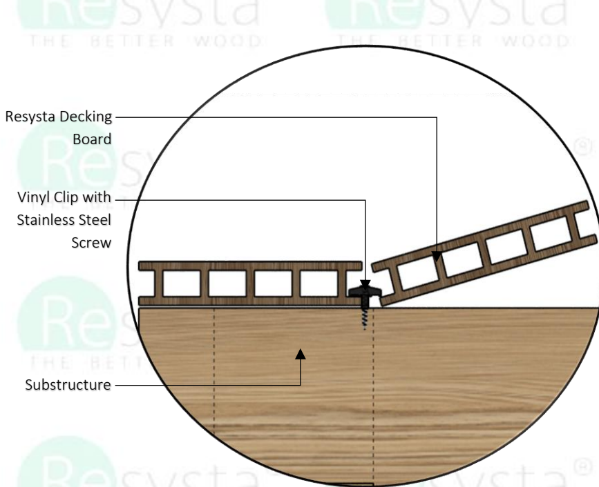
SECTION RESYSTA DECKING
