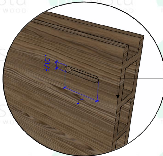
ISOMETRIC VIEW RESYSTA DECKING
