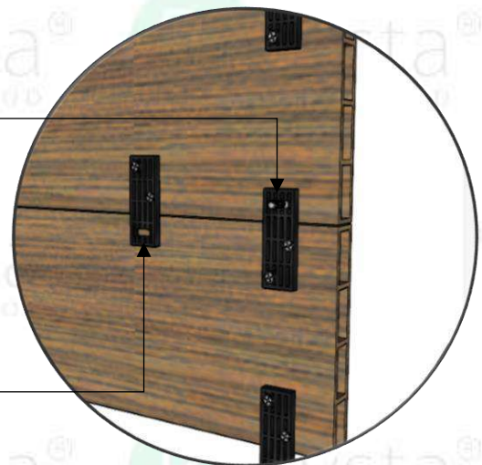
REAR ISOMETRIC VIEW Horizontal Wall Cladding Details
