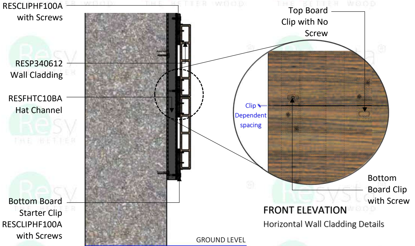
SIDE ELEVATION Horizontal Wall Cladding Details
