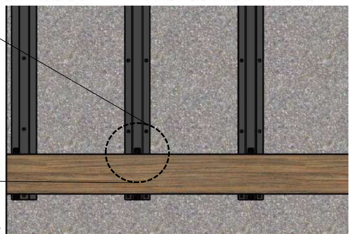
FRONT ELEVATION Horizontal Wall Cladding Details
