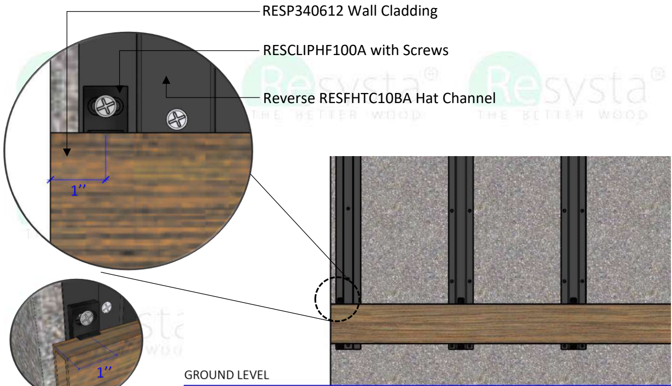
FRONT ELEVATION Horizontal Wall Cladding Details
