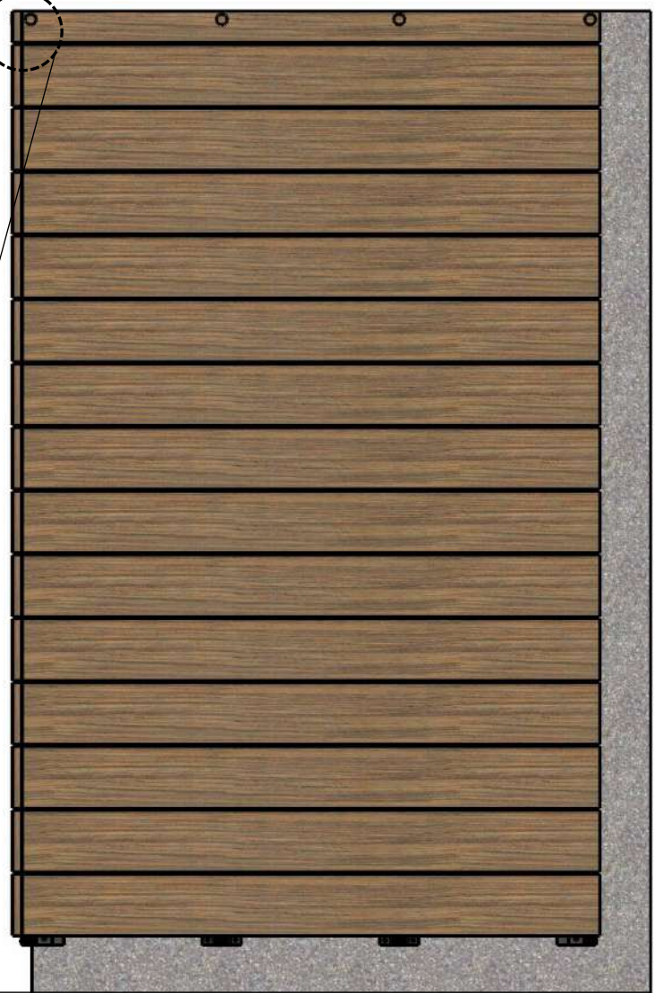
FRONT ELEVATION Horizontal Wall Cladding Details
