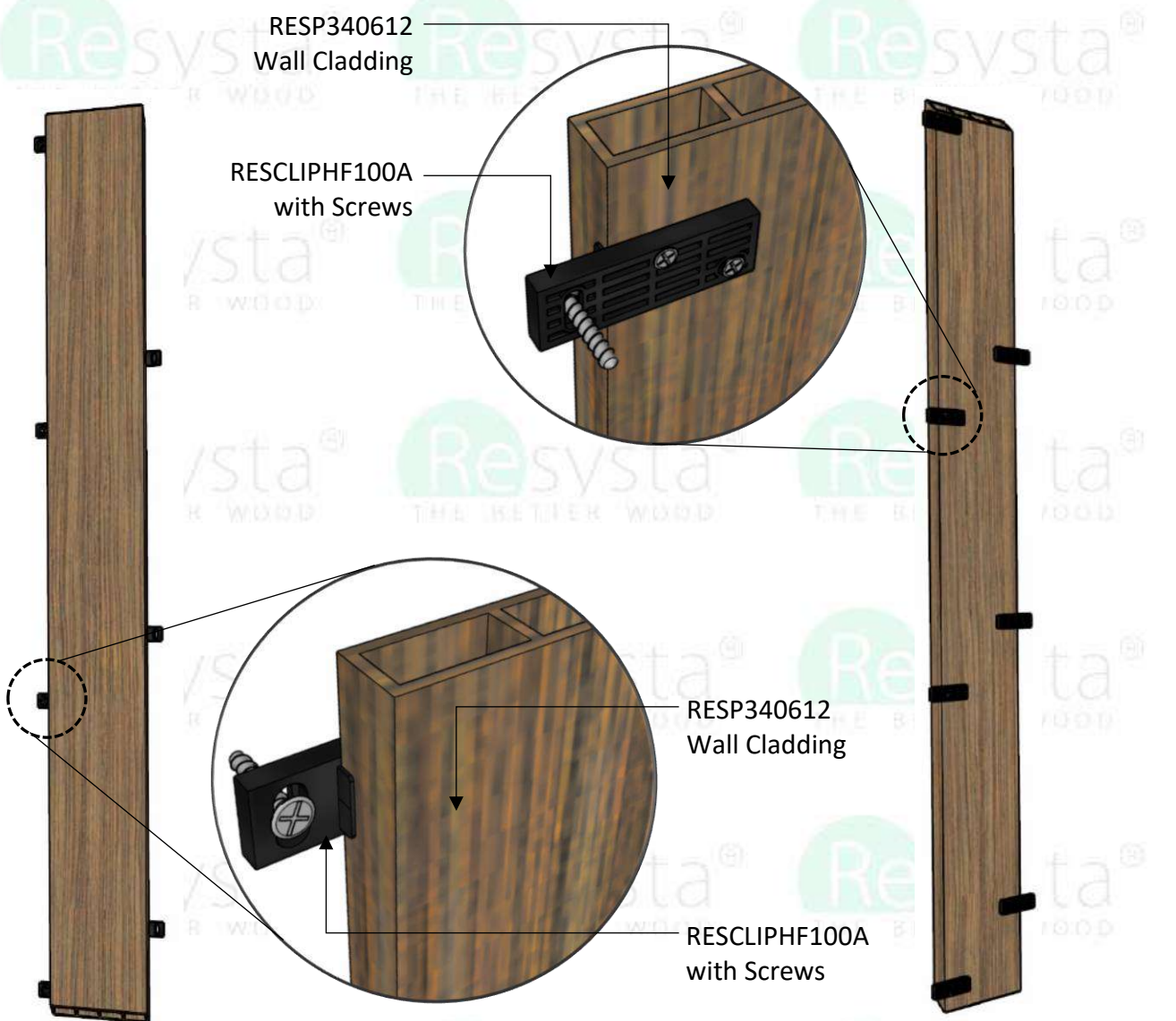
FRONT ISOMETRIC VIEW Vertical Wall Cladding Details
