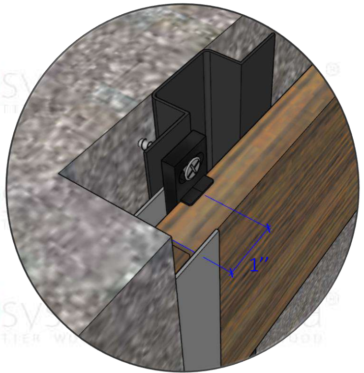
ISOMETRIC VIEW
