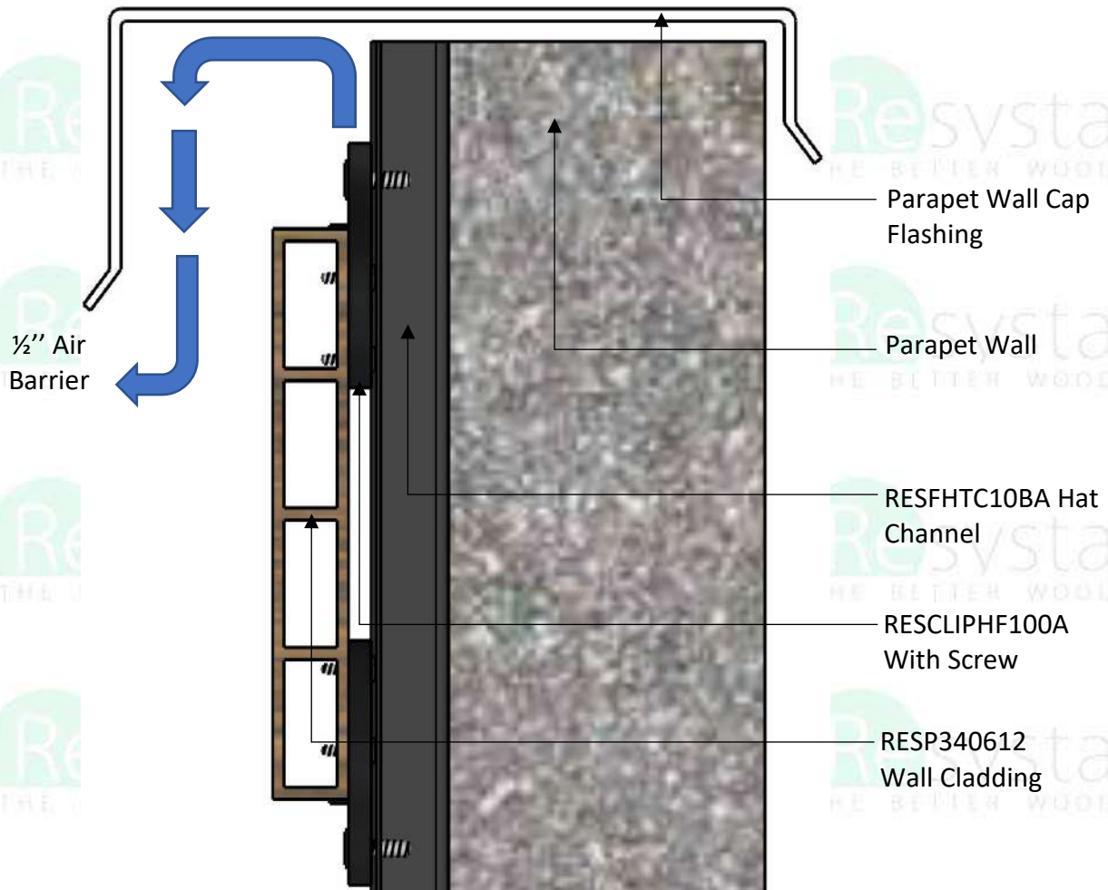
SECTION Wall Cladding Details
