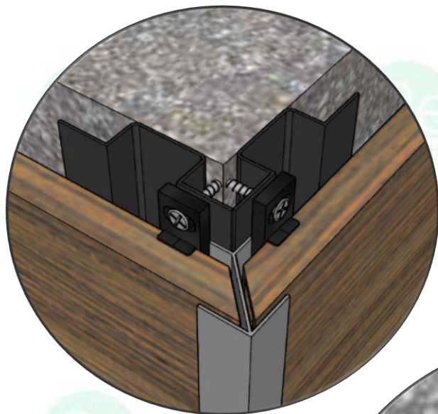
ISOMETRIC VIEW Horizontal Outside Corner
