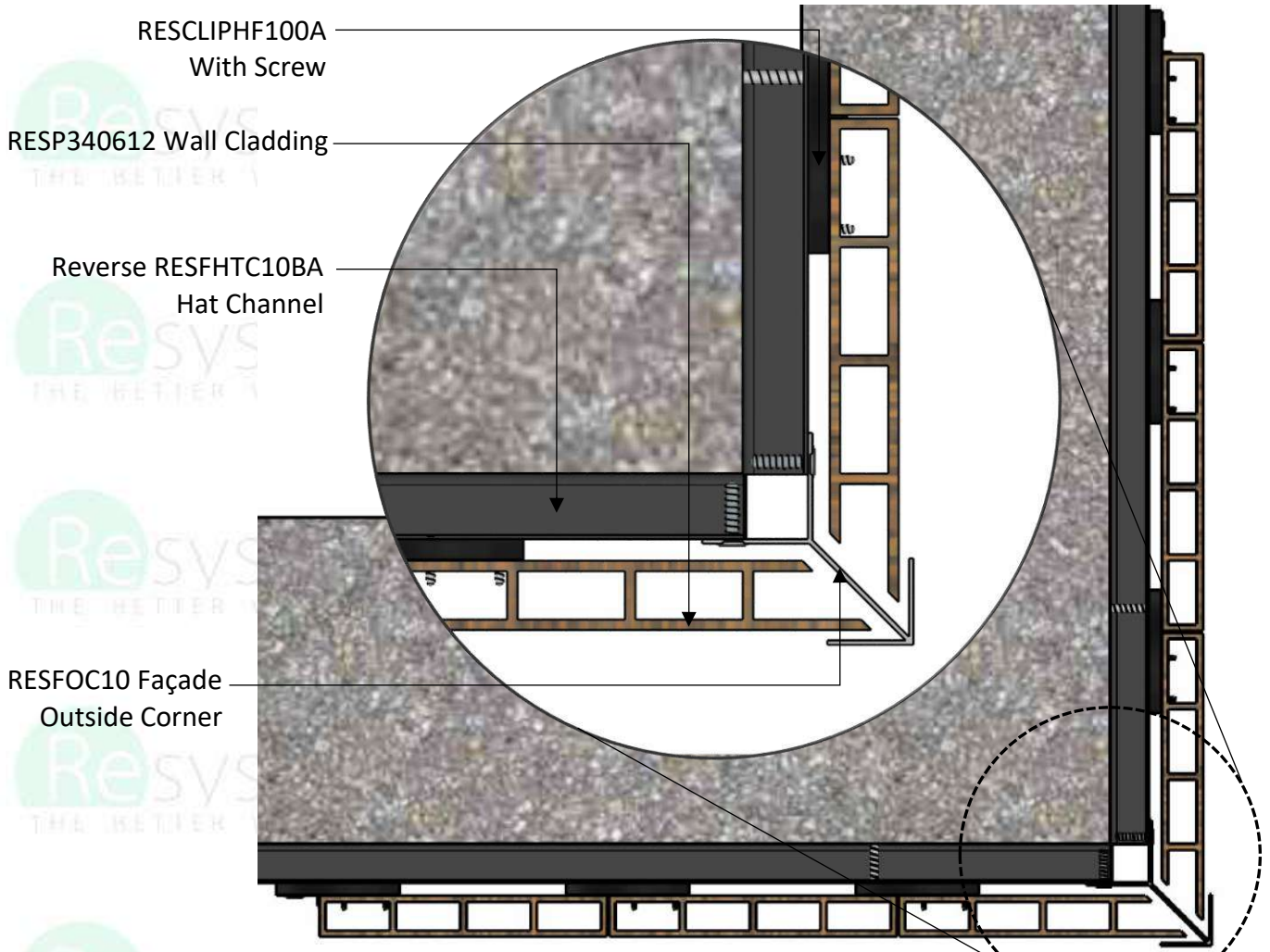
TOP VIEW Wall Cladding Vertical Outside Corner
