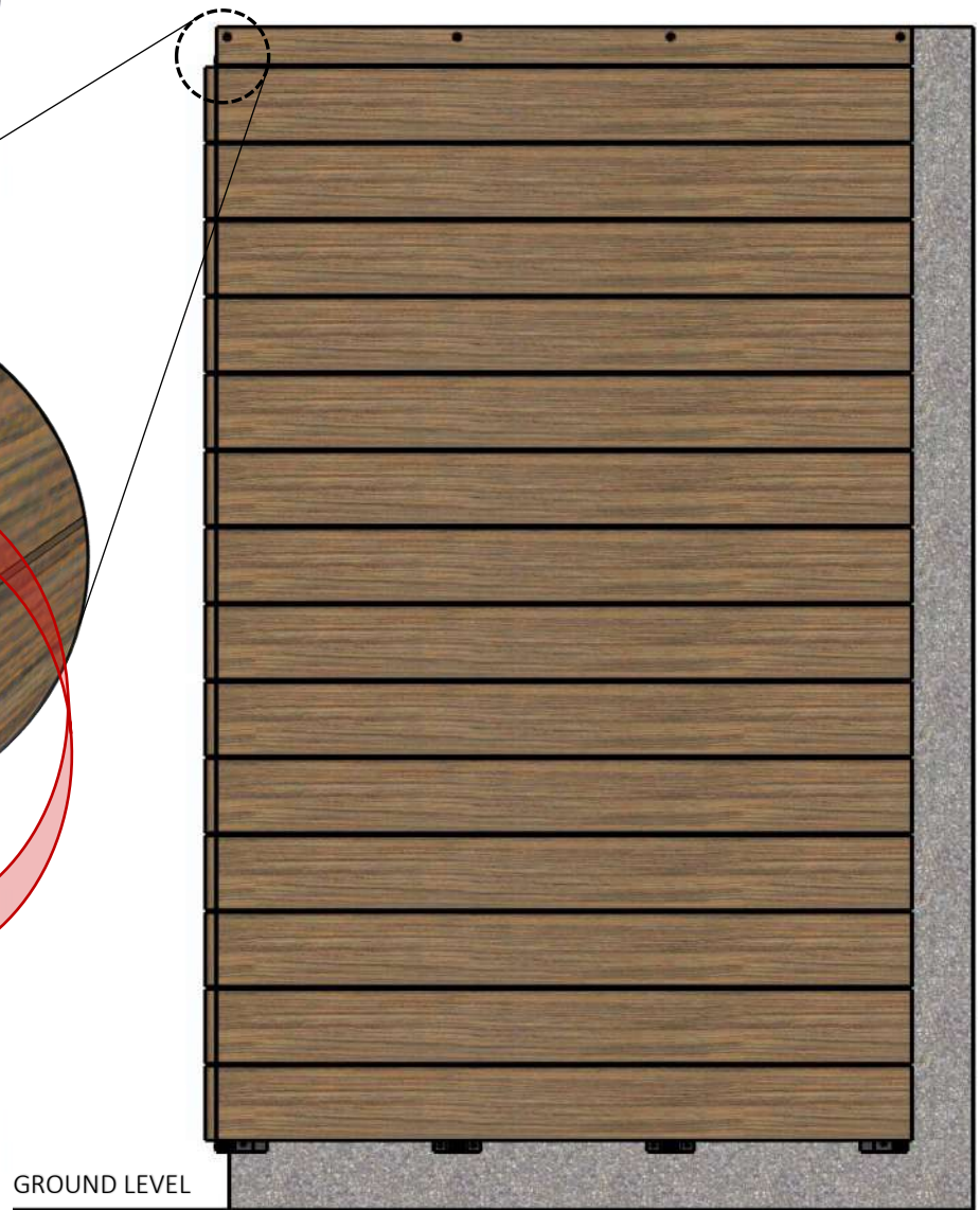
FRONT ELEVATION
