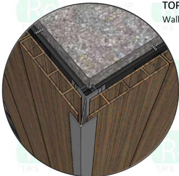
ISOMETRIC VIEW Wall Cladding Vertical Outside Corner
