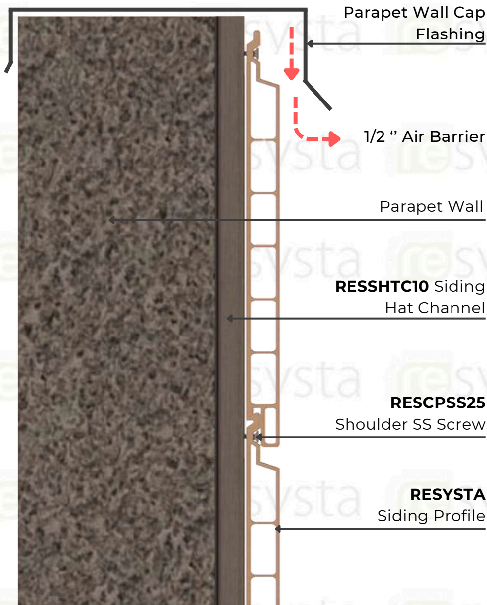
SECTION Quik-Trim System
