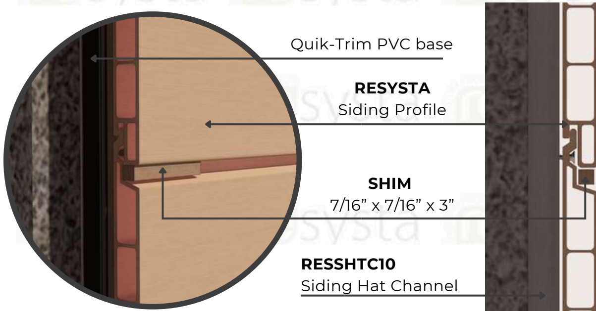
SECTION Quik-Trim System
