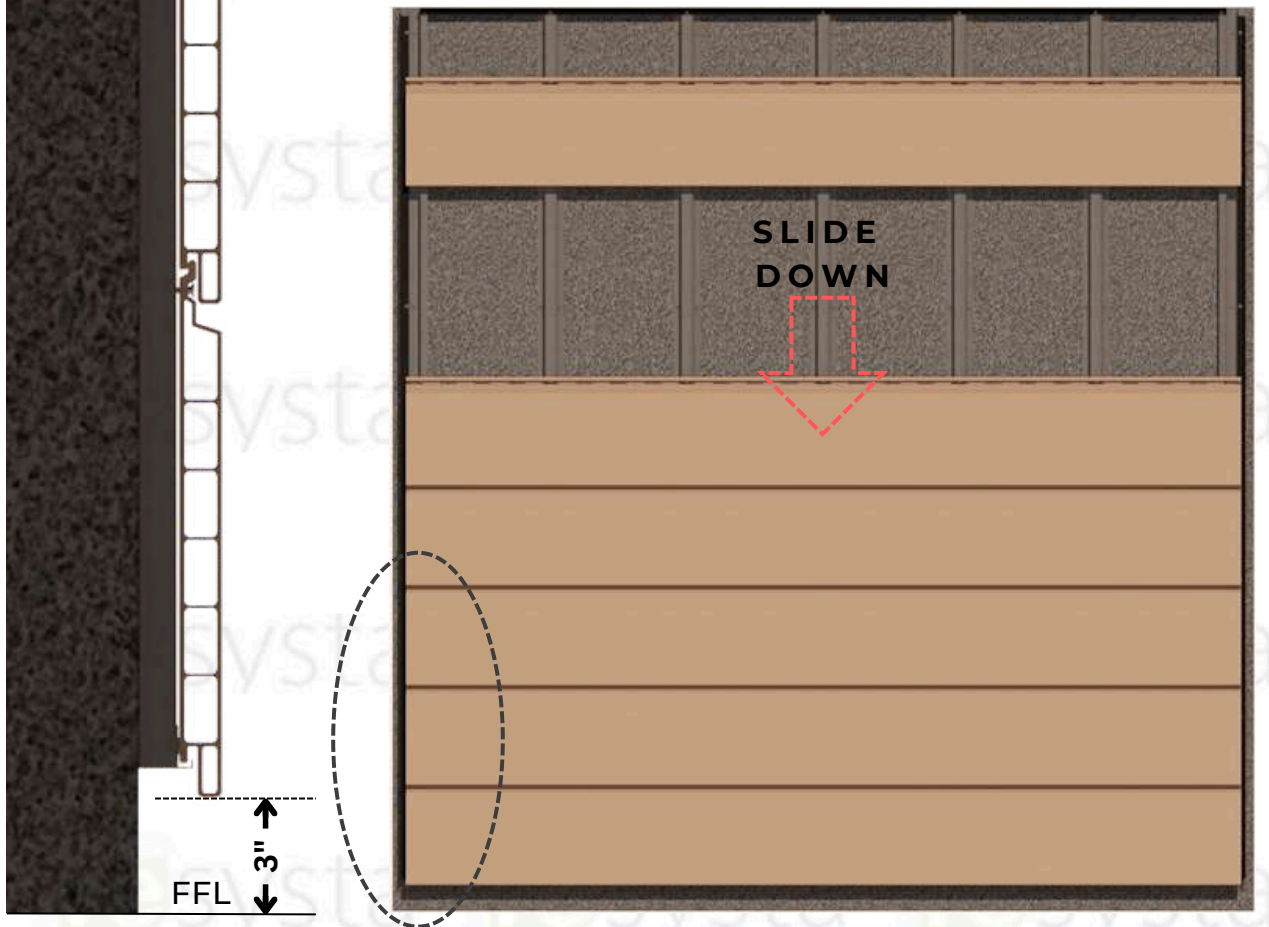
SECTION Quik-Trim System
