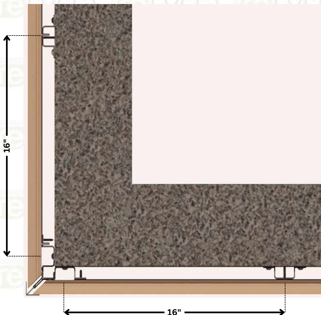
TOP VIEW Outside Corner
